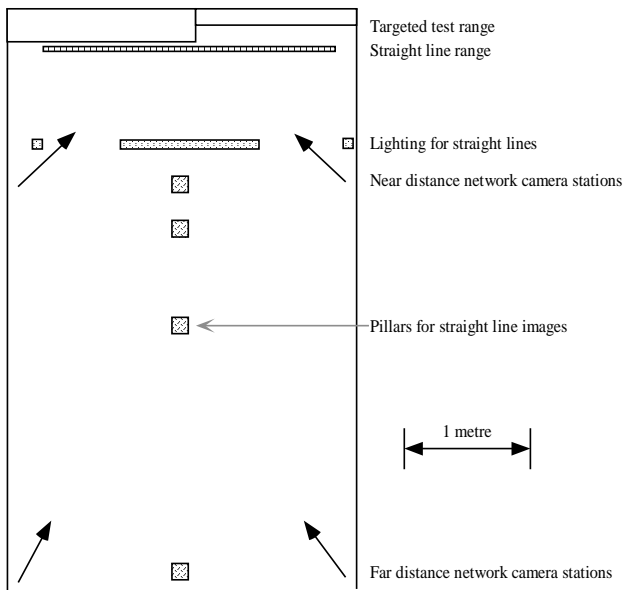
Figure 1. Layout of the calibration range.
