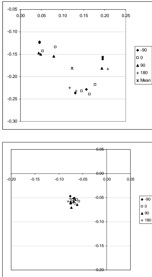
Figure 2. Inferred movement of the principal point for the RMIT EOS300D with the Canon zoom lens (top) and the Canon 24mm fixed lens (bottom).
