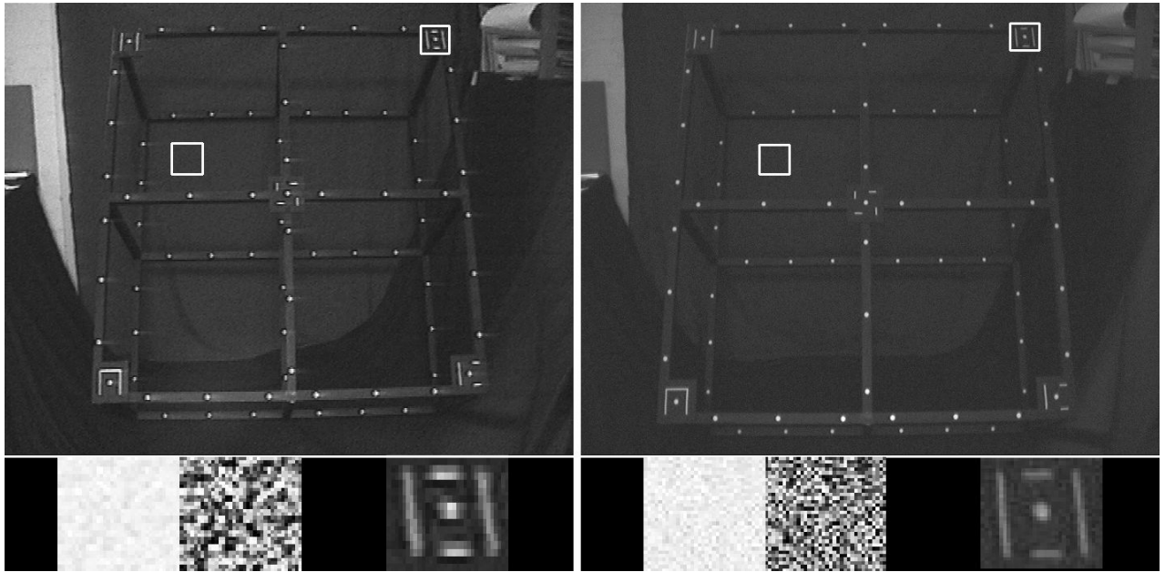
Figure 13. Comparison of images from the Hi8 (left) and digital (right) cameras. The inset images for each type of camera show enlarged sections of, from left to right, enhanced noise, histogram-equalised noise and a coded target. The noise and coded target regions used are indicated on the main images by the white outlines.
