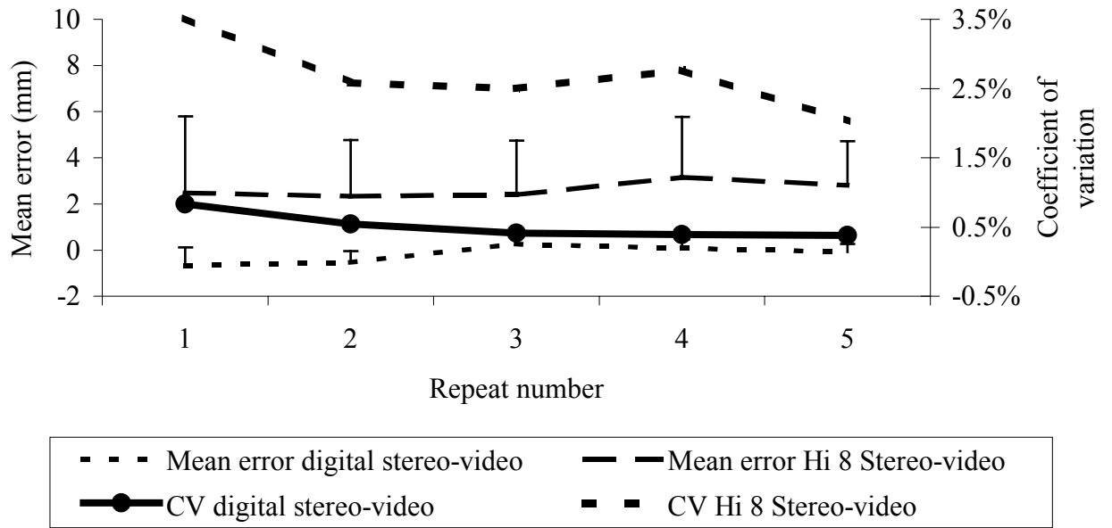
Figure 11. The effect of increasing the number of repeat measurements on optimising the accuracy and precision of measurements from digital and Hi8 stereo-video systems. Error bars indicate \pm 1 standard error.
