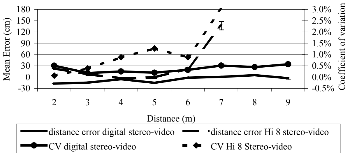
Figure 7. The accuracy and precision of distance measurements with a digital stereo-video system and a Hi8 stereo-video system. Error bars indicate \pm 1 standard error.
