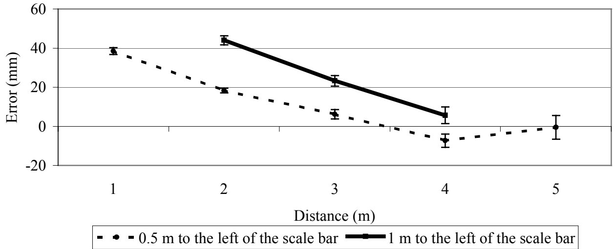
Figure 5. The effect of increasing the perpendicular distance of the silhouette from a scale bar on the accuracy and precision of measurements from a single camera system. Error bars indicate \pm 1 standard error.
