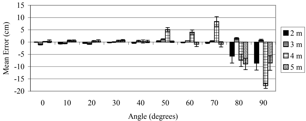
Figure 8. The effect of the increasing angle of the subject, relative to the camera system on the accuracy and precision of length estimates made with (a) a digital stereo-video and (b) a Hi8 stereo-video. Error bars indicate \pm 1 standard error.
