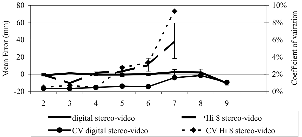
Figure 6. The accuracy and precision of length measurements with a digital stereo-video system and a Hi8 stereo-video system. Error bars indicate \pm 1 standard error.
