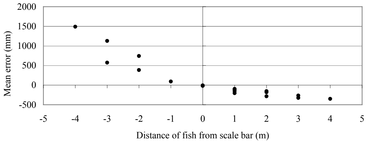
Figure 4. The affect of the position of the silhouette relative to the point of scaling on the accuracy of measurements of the length of a silhouette. Negative distances indicate that the plastic silhouette was in front of the scale bar. Fewer measurements were made when the silhouette was in front of the scale bar because the silhouette often blocked the view of the scale bar.
