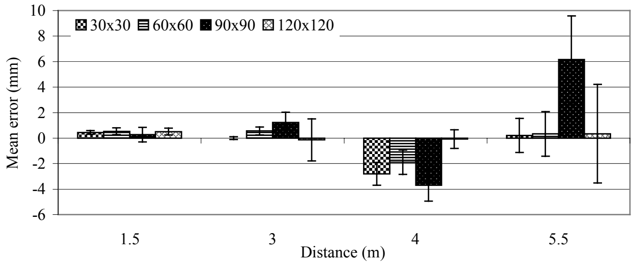
Figure 12. The effect of the ratio of pixels displayed in the variable zoom window on the accuracy and precision of length estimates. Error bars indicate \pm 1 standard error.
