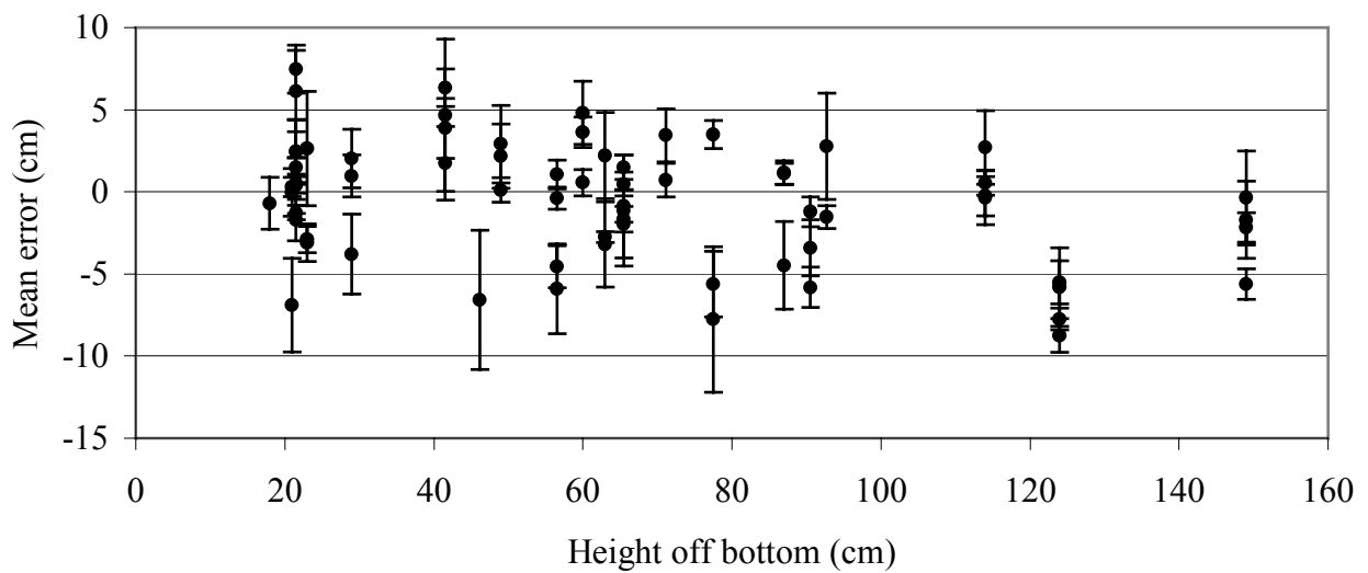
Figure 10. The effect of increasing the angle of the position of the silhouette in the height dimension of the field of view on the accuracy and precision of digital stereo-video measurements. Error bars indicate \pm 1 standard error.
