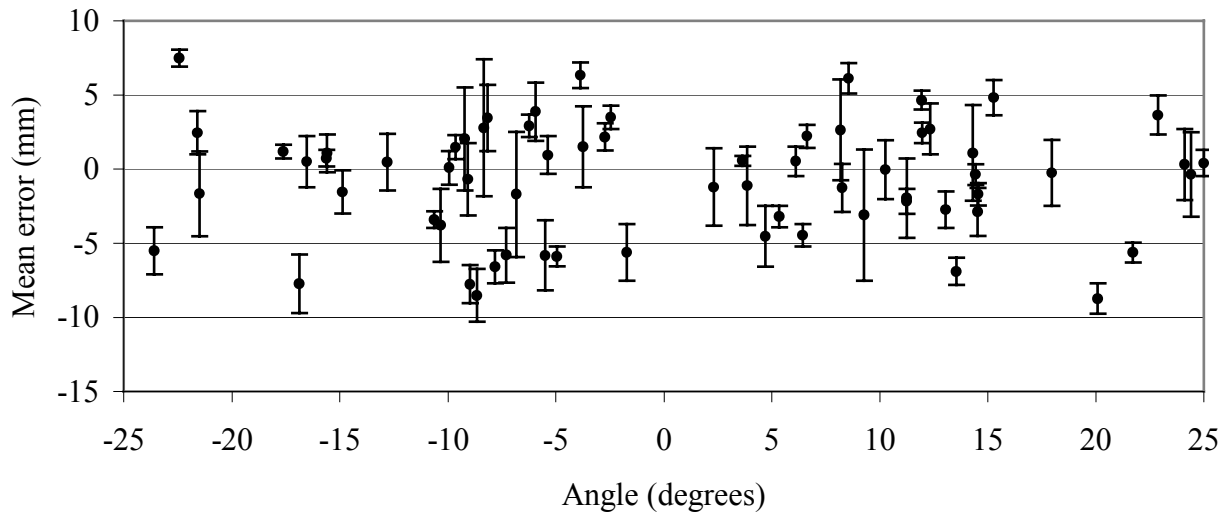
Figure 9. The effect of increasing the angle of the position of the silhouette in the width dimension of the field of view on the accuracy and precision of digital stereo-video measurements. Error bars indicate \pm 1 standard error.
