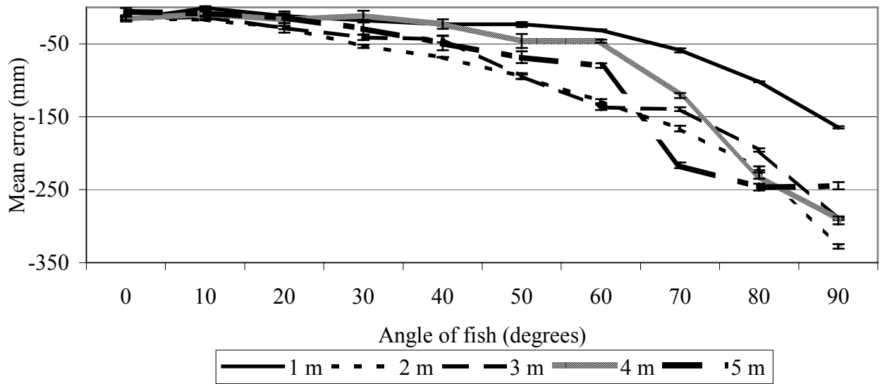
Figure 3. The effect of increasing angle of the silhouette on the accuracy and precision of single video camera measurements. Error bars indicate \pm 2 standard errors.
